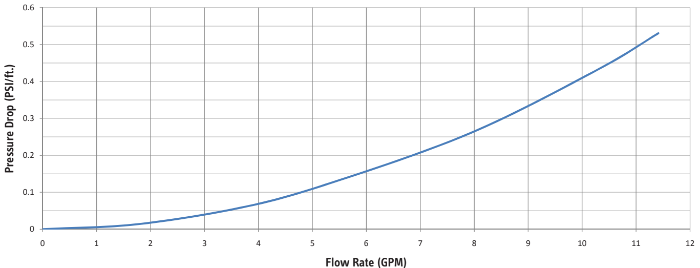
DN 20 Stainless Steel Hose Pressure Drop Curve
