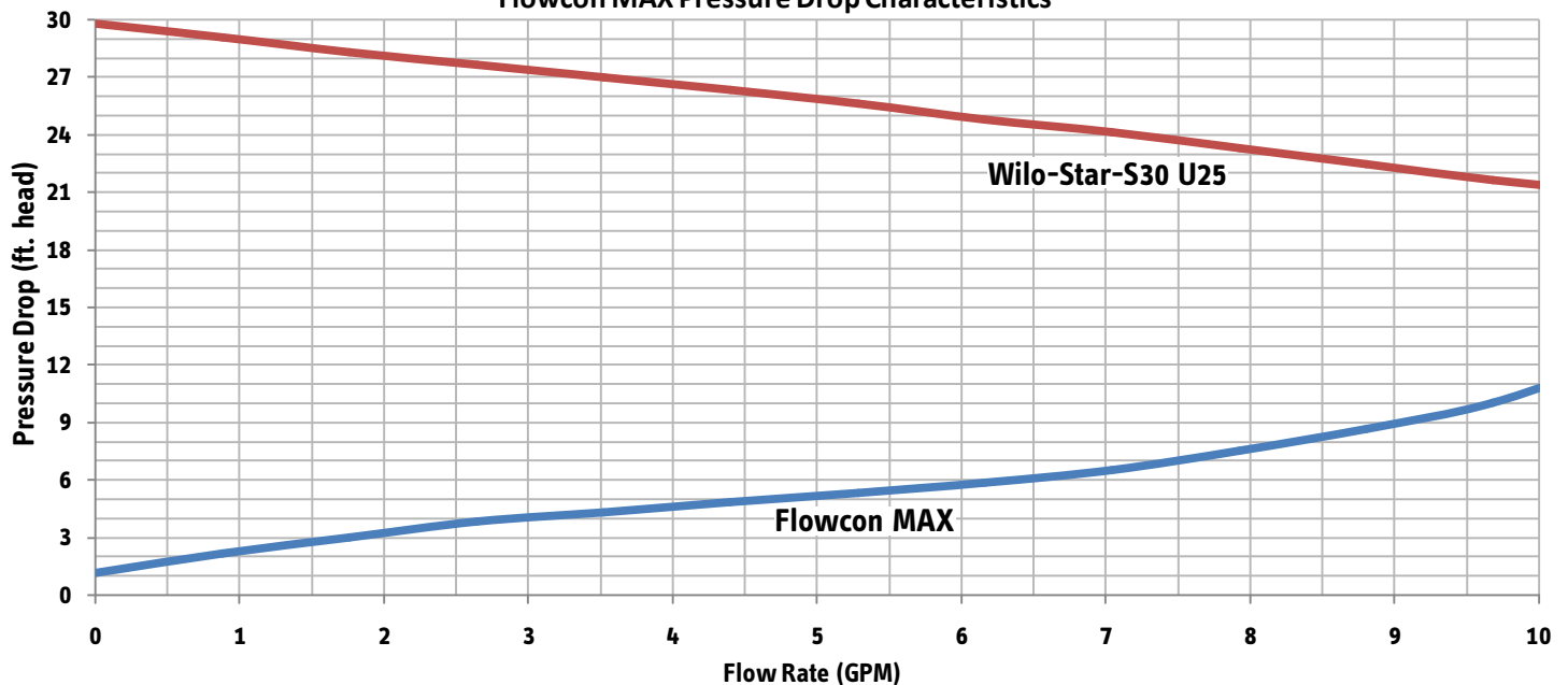
Flowcon MAX Pressure Drop Characteristics
