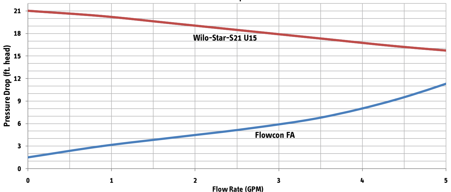
Flowcon FA Pressure Drop Characteristics
